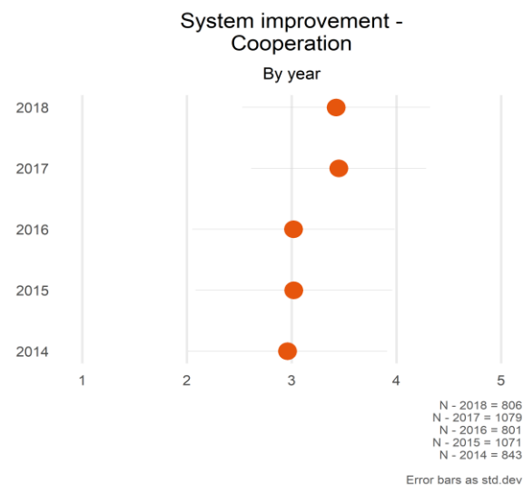
Figure 11: System improvement – cooperation score, all participating countries by year
